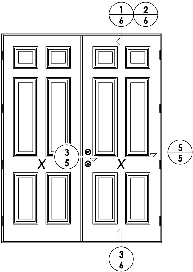
ELEVATION (XX)
