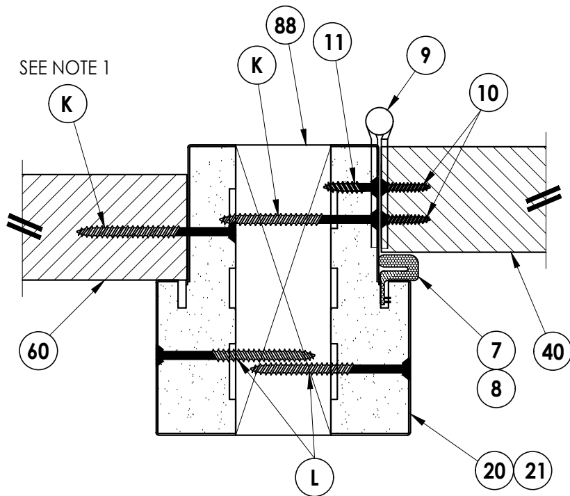
2 5 HORIZONTAL CROSS SECTION
