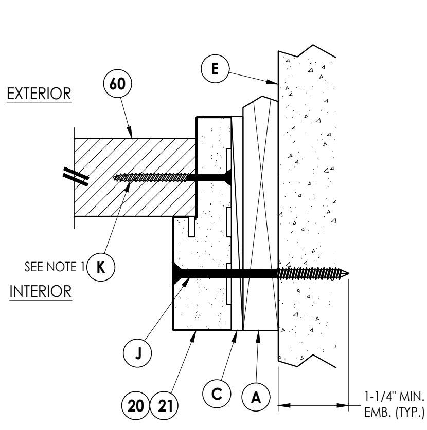
4 5 HORIZONTAL CROSS SECTION Shown w/1X sub-buck
